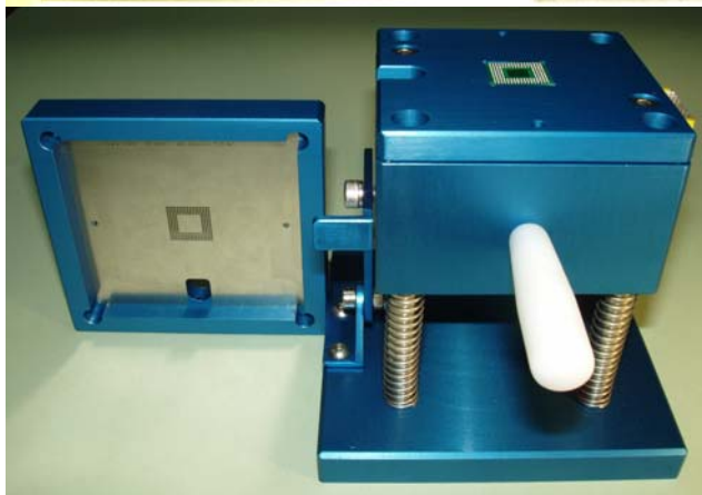
Stapula for BGA paste/flux application. 19cm length
